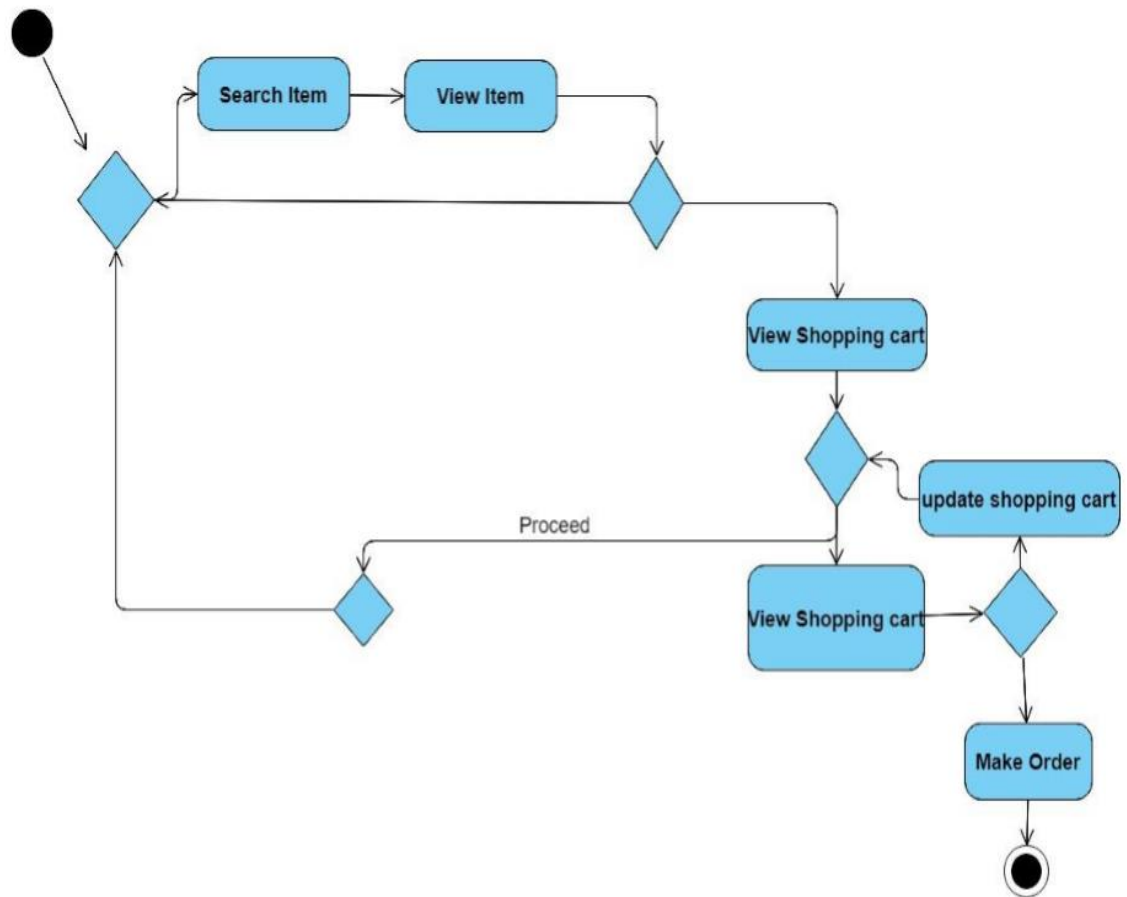
Figure 3: Activity Diagram
