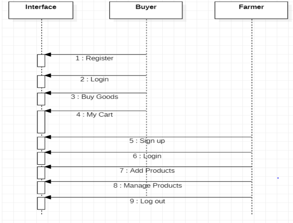
Figure 2:Sequence Diagram
