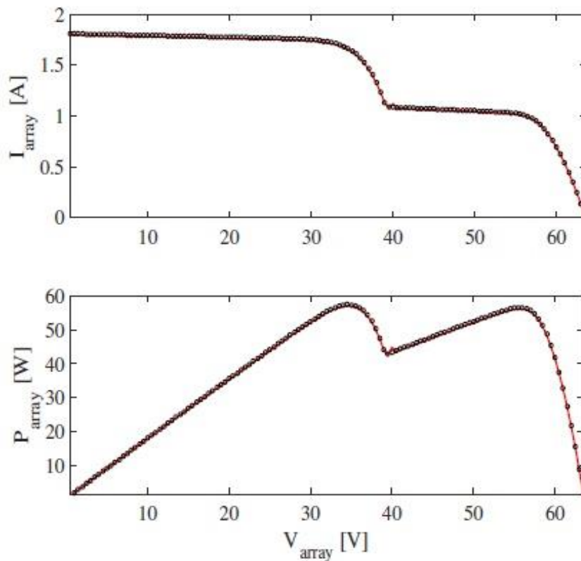
Fig. 5: Current-Voltage (V-I) & Power-Voltage (P-V) characteristic of TCT configuration
