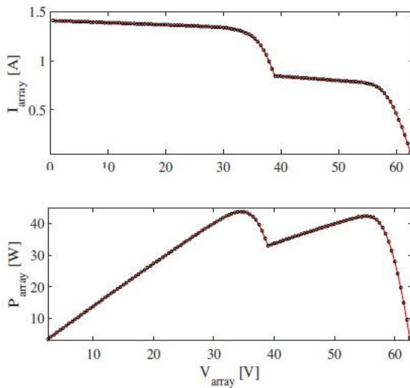
Fig. 4: Current-Voltage (V-I) & Power-Voltage (P-V) characteristic of SP configuration
