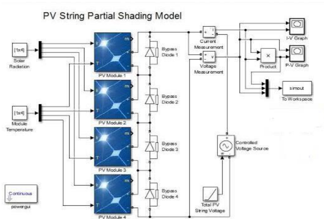
Fig.3: Simulation in MATLAB/Simpower
