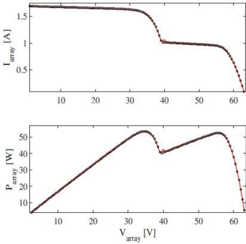
Fig. 6: Current-Voltage (V-I) & Power-Voltage (P-V) characteristic of BL configuration.
