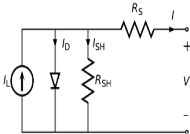
Fig. 2: Equivalent circuit of PV cell
