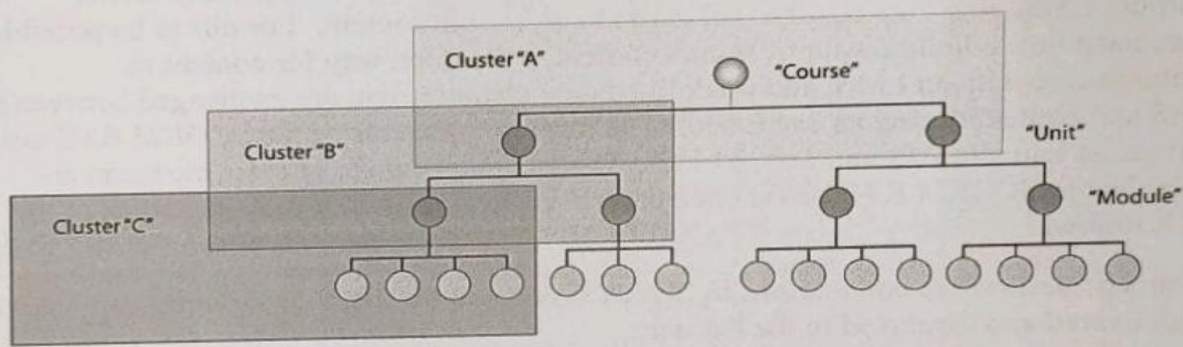
Figure 1.3.5a: Conceptual Activity Tree and Clusters
