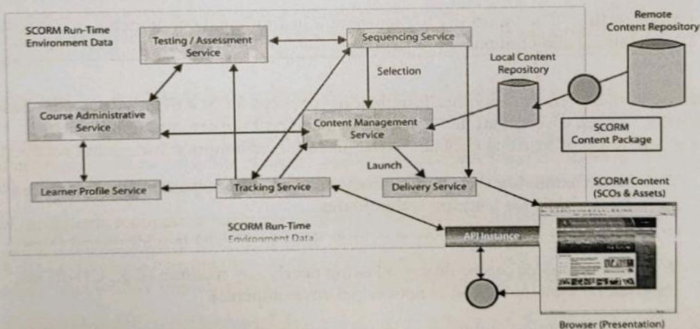
Figure 1.2.2a: Highly generalized model of an LMS
