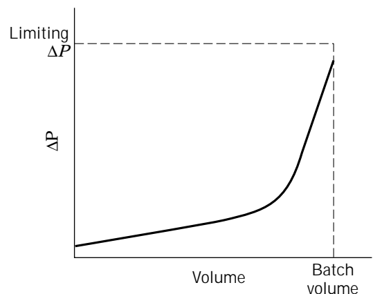
Figure 16. Example of an ideal filtration system. Adapted from "Engineering Considerations in Sterile Filtration Processes" by Holly Haughney in Sterile Pharmaceutical Products: Process Engineering Applications , edited by Kenneth E. Avis. Copyright © 1995 by Interpharm Press, Inc. All rights reserved. Adapted by permission.
