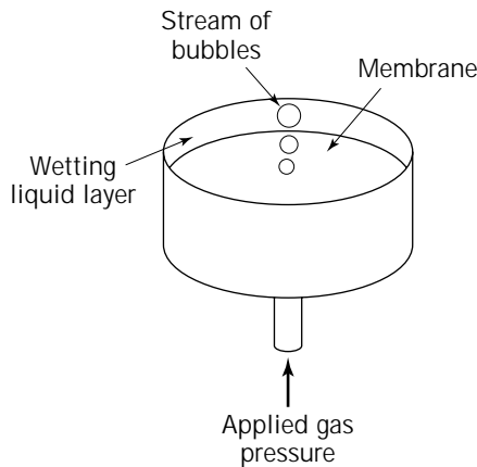
Figure 8. Bubble point test. Courtesy of Pall Corporation (20).
