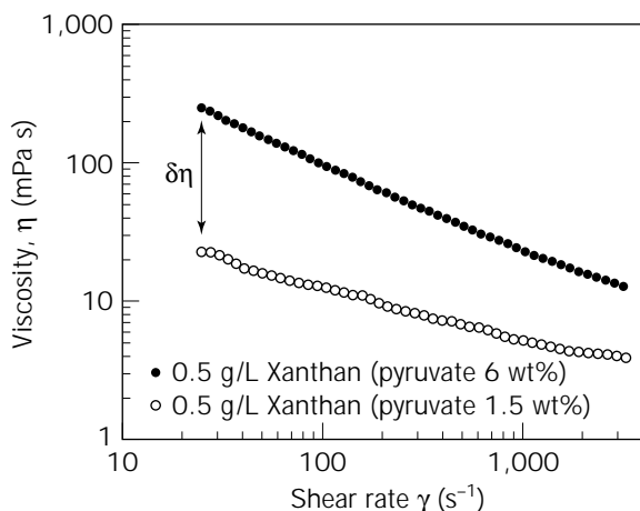
Figure 12. Comparative viscosity curves of 0.5 g/L xanthan in 0.12 M KCl with varying degree of pyruvate substitution. Filled symbols correspond to xanthan with about 6 wt% pyruvate content and M_w of 7 \times 10^6 g/mol; open symbols relate to xanthan with about 1.5 wt% pyruvate content and M_w of 6.5 \times 10^6 g/mol (run F7). Source: Results from Flores-Candia (21).
