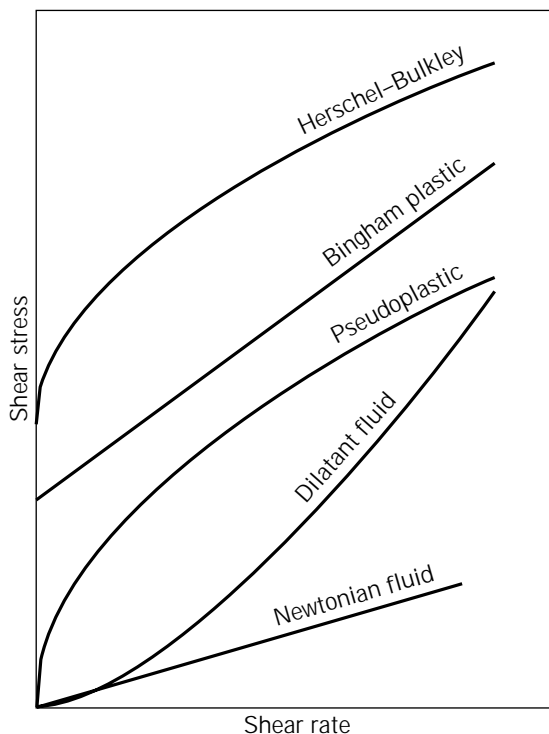
Figure 1. Rheological models.
