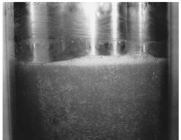
Figure 10. Mixing and mass transfer challenges in pullulan fermentation. The picture is taken when the agitator equipped with Rushton turbines is rotating at 500 rpm. The layer of fermentation broth adjacent to the fermenter wall remains stagnant with trapped air bubbles.
