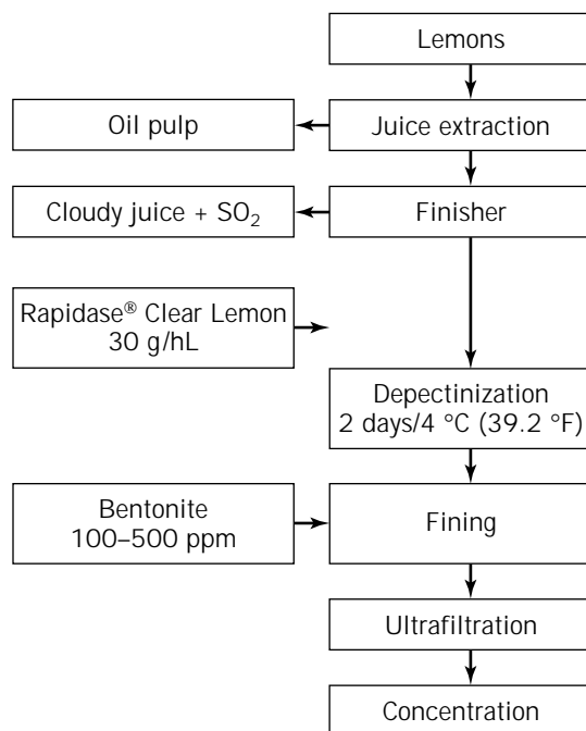
Figure 25. Lemon juice process.
