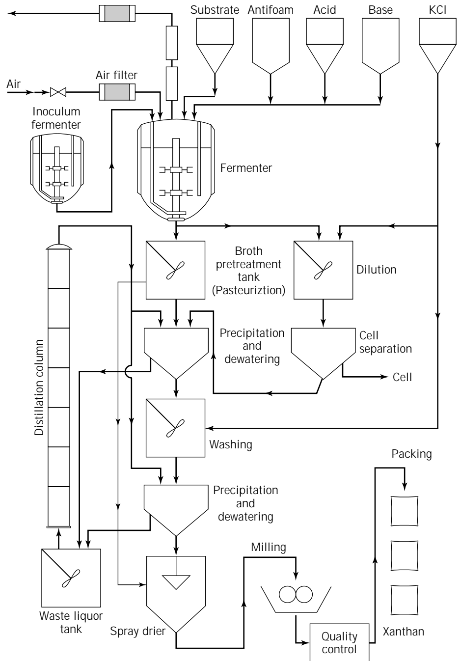
Figure 5. Flowsheet for production of xanthan.
