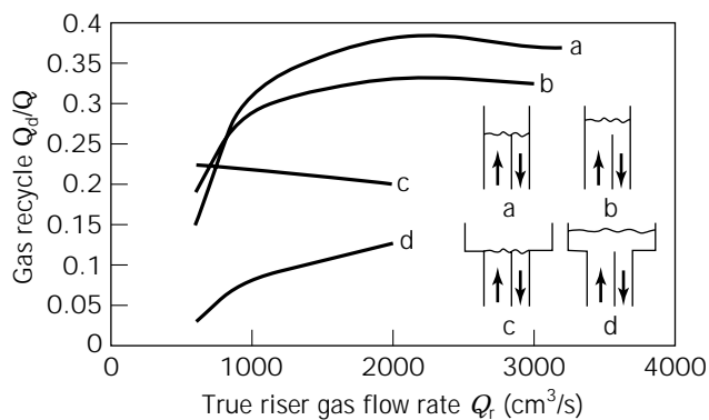
Figure 16. Gas recirculation in a split-cylinder ALR. The level indicated corresponds to no-aeration conditions. Adapted from Siegel et al. (35).
