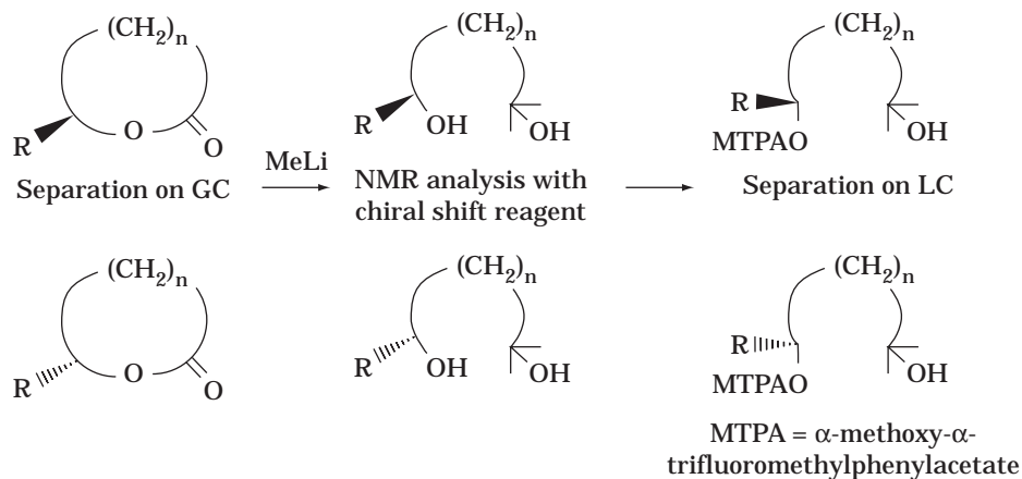
Scheme 4. Determination of enantiomeric excesses of lactones.
