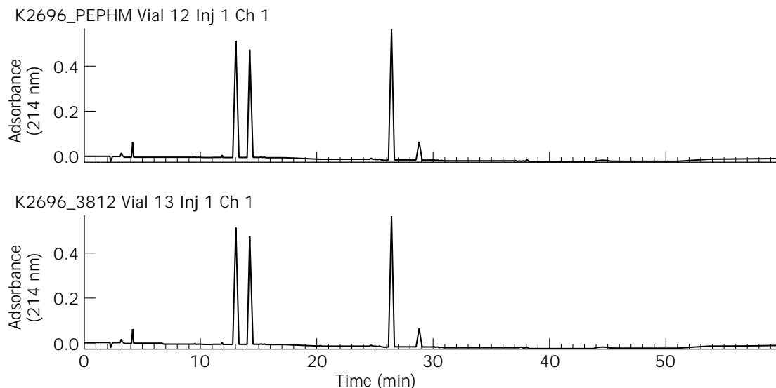
Figure 6. Peptide map of insulin sample (bottom panel) compared to a human insulin reference standard (top panel). Column: Lichorsorb RP-18, 5 \mu m; solvent A: 0.2 M sodium sulfate, 0.04 M phosphoric acid in 10% acetonitrile, pH adjusted to 2.5 with ethanolamine; solvent B: 50% acetonitrile; flow rate: 1.0 mL/min; temperature: 40 ^{\circ} C; 25 \mu g of sample was cleared prior to injection and eluted with a gradient.
