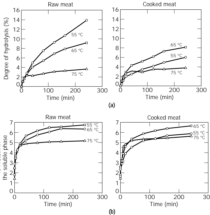
Figure 22. (a) Hydrolyses curves (osmometer) at 8% beef, protein. enzyme, Esperase 7.5 FG, dosage 0.5% of protein, —○—, 55 °C; —□—, 65 °C; —△—, 75 °C. (b) Solubilization of protein by hydrolyses of beef; meat, enzyme, Esperase 7.5 FG; dosage, 2.0 kg/t bone.
