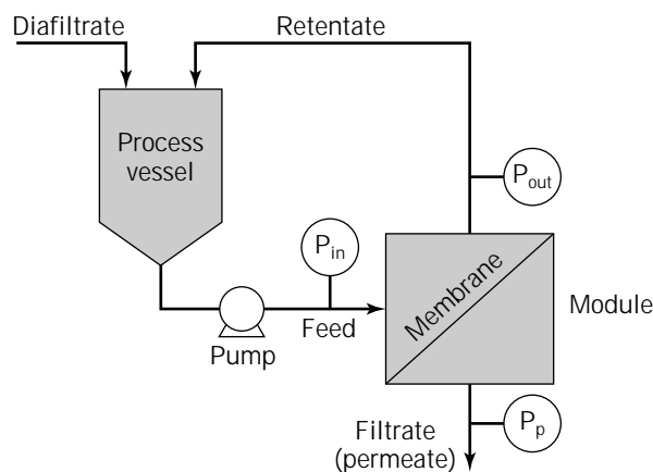
Figure 8. Schematic of a tangential-flow filtration operation (clarification, concentration, and diafiltration).
