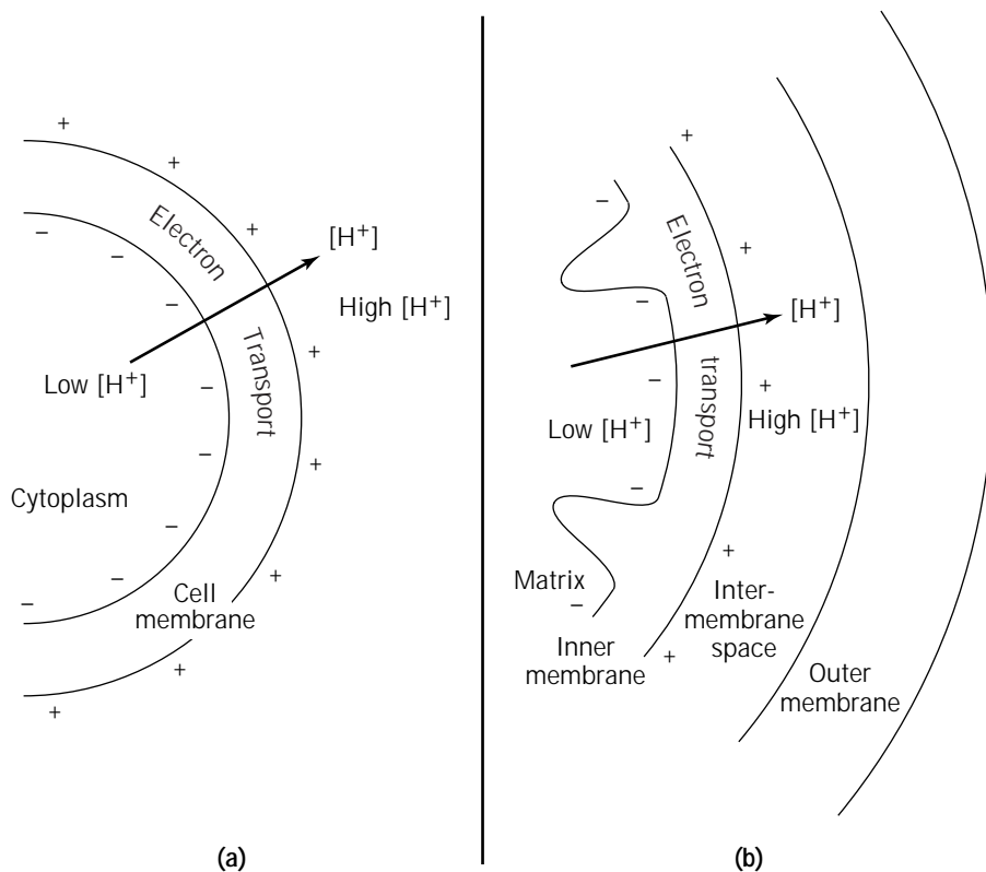
Figure 1. Electron transport in bacterial cell membranes (a) and mitochondrial membranes (b) result in proton translocation accompanied by a membrane potential (outside positive) and a pH gradient (outside acidic). The molecular mechanisms and the intermediates are not shown.
