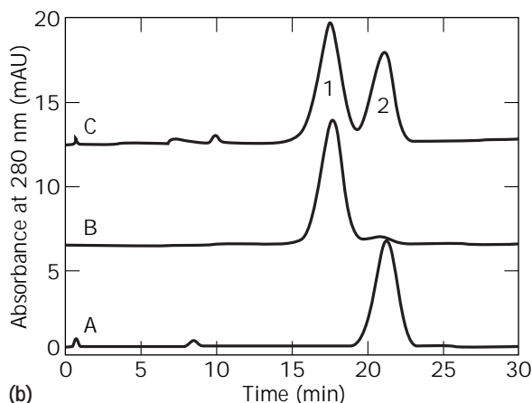
Figure 1. (a) Strong cation exchange chromatography on a sulfopropyl column (TSK SP 5PW, 75 mm × 7.5 mm i.d.) of three samples: A, rhDNase; B, its deamidated variant; and C, a mixture of the two variants. (b) Cation exchange chromatography of three samples: A, rhDNase; B, its deamidated variant; and C, a mixture of the two variants on a tentacle ion exchanger (LiChrosphere SO 3 - 50 mm × 4.6 mm i.d.). The two sets of chromatograms were obtained under the same chromatographic conditions. (Source: Reproduced with permission from Ref. 28.)
