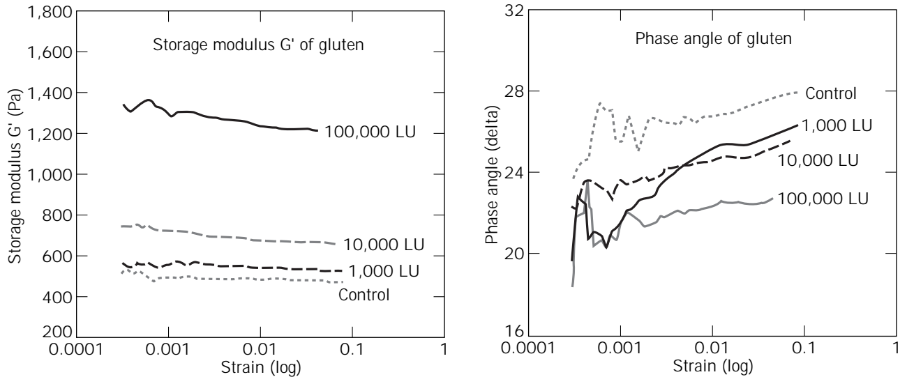
Figure 10. The effect of lipase on the rheological properties of gluten.
