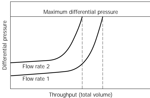
Figure 15. Comparison of a filtration performed with different flow rates. Adapted from "Engineering Considerations in Sterile Filtration Processes" by Holly Haughney in Sterile Pharmaceutical Products: Process Engineering Applications , edited by Kenneth E. Avis. Copyright © 1995 by Interpharm Press, Inc. All rights reserved. Adapted by permission.
