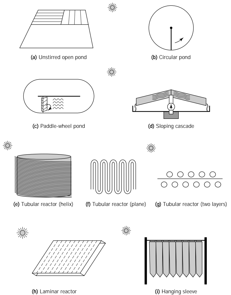
Figure 2. Illustration of algal mass culture systems.
