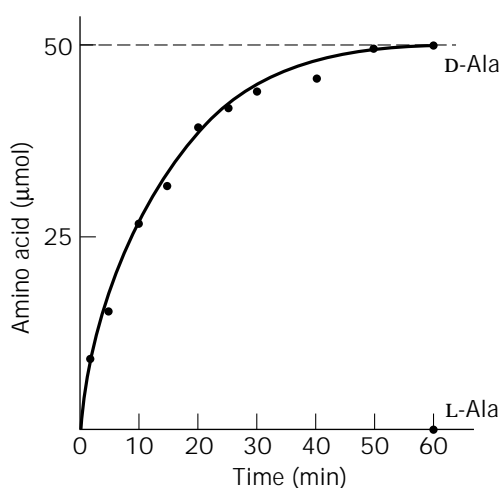
Figure 1. Kinetic resolution of DL-alanine amide by O. anthropi D-aminopeptidase. A reaction mixture containing 0.5 mmol tris(hydrochloride), pH 8.0, 0.1 mmol DL-alanine amide hydrochloride, and 5 units of the purified enzyme in a total volume of 5.0 mL was incubated at 30 °C. The content of L-alanine was measured by L-alanine dehydrogenase.
