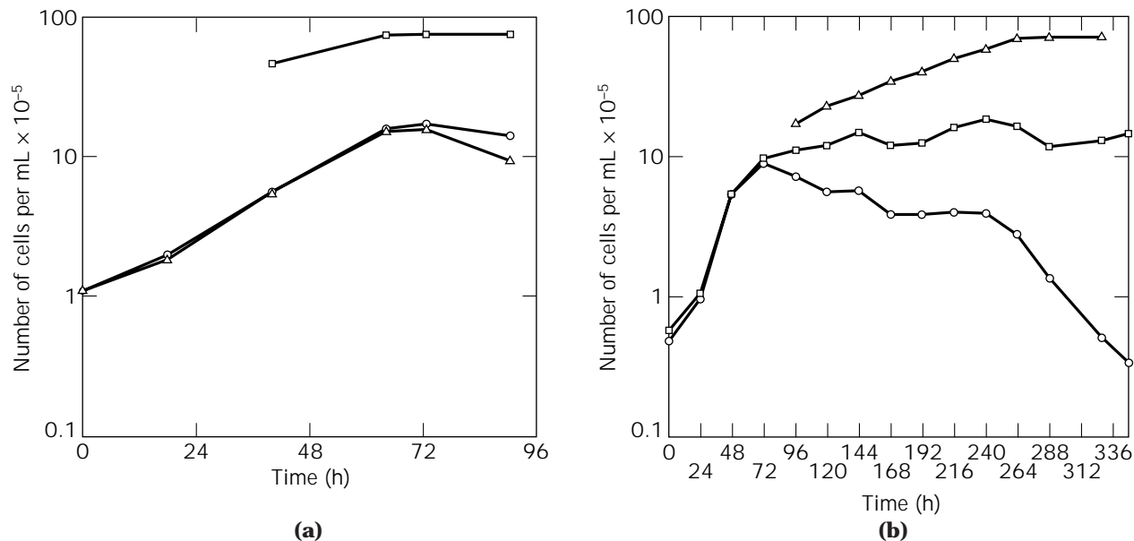
Figure 5. Growth curves and MAb production by two hybridoma lines (a, XMMME-C, and b, XMMEN-A) with growth-associated and non-growth-associated productivity patterns. Total (○), viable (Δ), and MAb concentration per mg/L (□).
