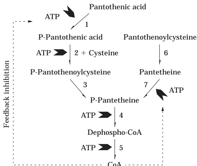
Figure 3. The pathway for the biosynthesis of coenzyme A from pantothenic acid, L-cysteine, and ATP. For chemical structures of each compound, see Table 1. CoA, coenzyme A.
