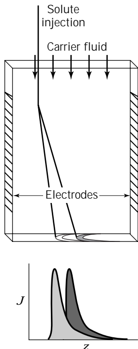
Figure 10. Schematic of the CFE showing electrode placement, multicomponent sample injection, carrier fluid flow, and product distribution. Typical elution bands are shown beneath the chamber corresponding to the two crescent-shaped bands on the lower surface of the chamber. The skewing is a deformation of the sample bands referred to as the crescent phenomena (2,40), which is caused by the interaction of hydrodynamic and electrokinetic effects.
