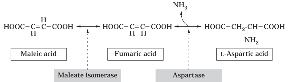
Figure 4. L-Aspartic acid formation from maleic acid
