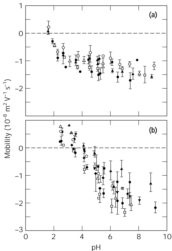
Figure 9. Electrophoretic mobility as a function of pH for bottom-fermenting strains (a) and top-fermenting strains (b) in 1 mM \text{KNO}_3 (45).
