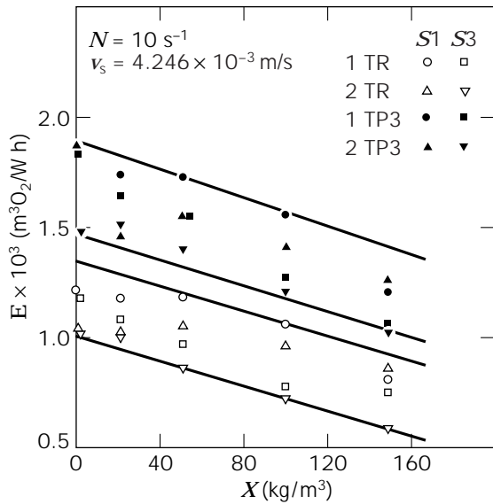
Figure 15. Relation between oxygen transfer efficiency and solid concentration for various agitators. (Source: From Ref. 35, with permission.)
