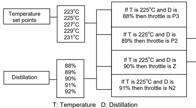
T: Temperature D: Distillation FIGURE 3.3.5:Fuzzy rules for the temperature set point 225°C
