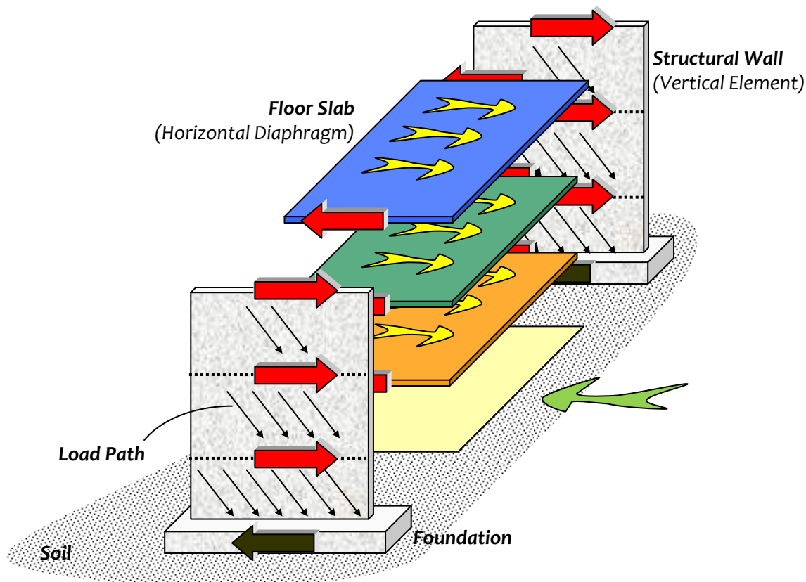
Figure 1.2: SEs create load path in each direction: Allow flow of inertia forces through them
