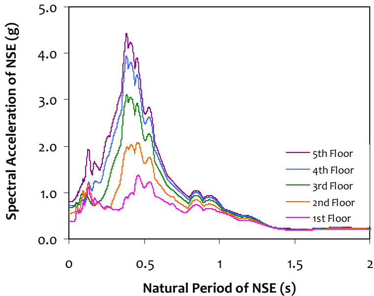
Figure 3.9: Floor Acceleration Response Spectra: Acceleration response of a spectrum of NSEs with different natural periods, but with the same damping (5% of critical) and subjected to the five different horizontal floor acceleration histories in a five storey RC building
