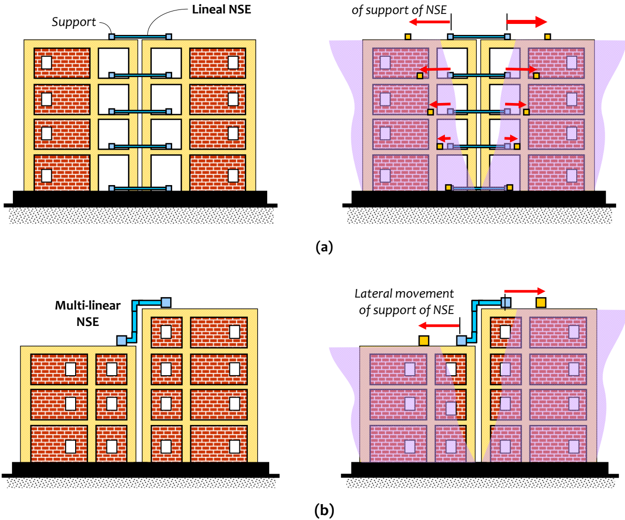
Figure 3.25: Relative Displacement between two items shaking independently on ground: Lineal NSEs need to sustain lateral and vertical displacements without failure: (a) connected to the same level on both parts of a building, and (b) connected to different levels on the two parts of a building
