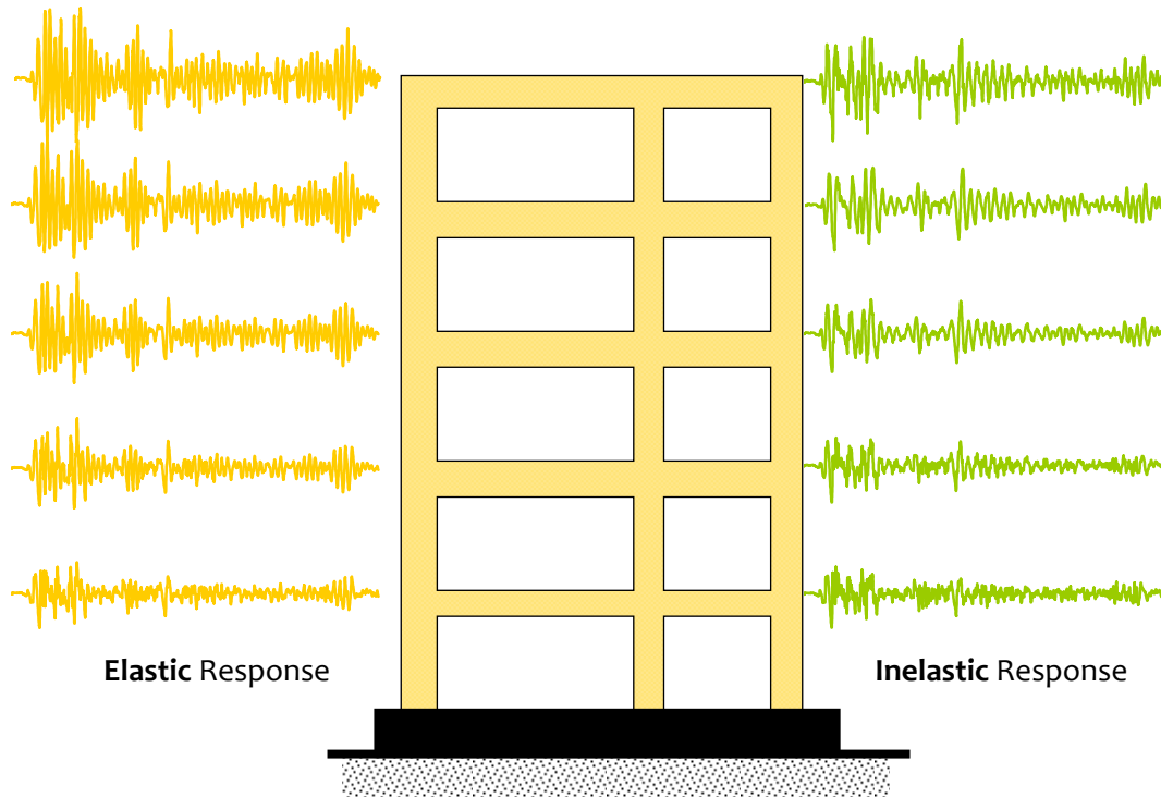
Figure 3.5: Floor Acceleration Response: Inelastic response significantly different from elastic response
