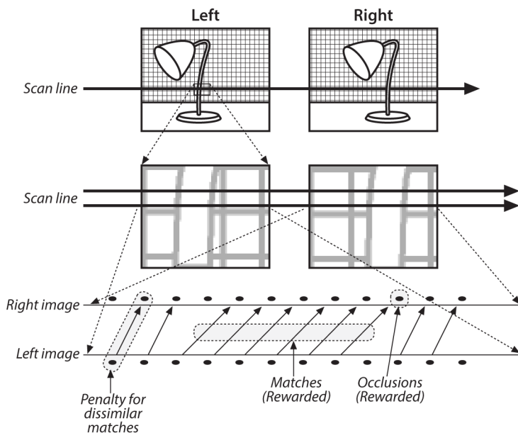
Figure 19-17. Stereo correspondence starts by assigning point matches between corresponding rows in the left and right images: left and right images of a lamp (upper panel); an enlargement of a single scan line (middle panel); visualization of the correspondences assigned (lower panel)
