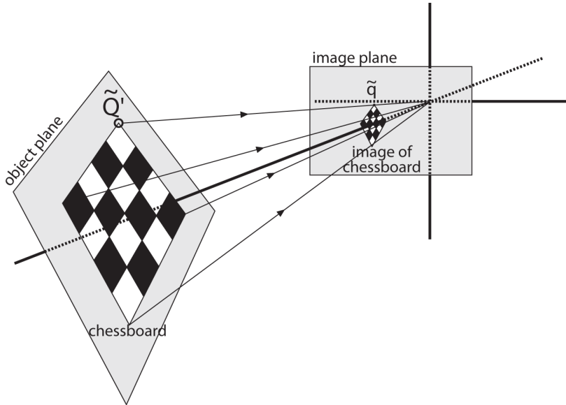
Figure 18-16. View of a planar object as described by homography: a mapping—from the object plane to the image plane—that simultaneously comprehends the relative locations of those two planes as well as the camera projection matrix
