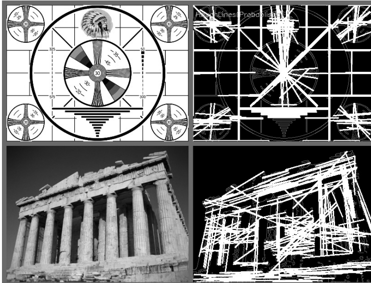
Figure 12-7. The Canny edge detector ( param1=50, param2=150 ) is run first, with the results shown in gray, and the progressive probabilistic Hough transform ( param1=50, param2=10 ) is run next, with the results overlaid in white; you can see that the strong lines are generally picked up by the Hough transform
