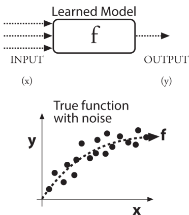
Figure 20-2. Setup for statistical machine learning: we train a classifier to fit a data set; the true model f is almost always corrupted by noise or unknown influences
