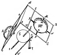
3.30 Cavendish's null experiment to show that electricity obeys the same law as gravity. From Cavendish, El. Res. (1879), 104.
