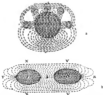
1.4 Cartesian magnetism, from Descartes, Principia (1644): (a) the earth's magnetic vortices ABFGE and BAEHF , with oriented lodestones at I , K , L , M , and N (b) the joint vortex TXVRVX of lodestones P and Q with opposite poles facing.
