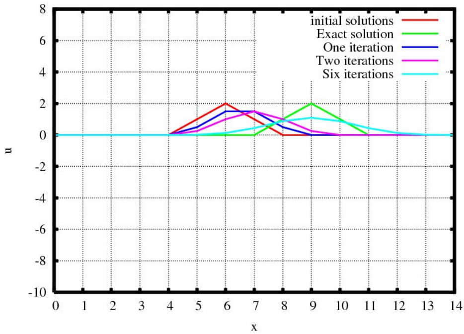
Figure 4-2: Solution using upwind scheme with Courant number 0.5
