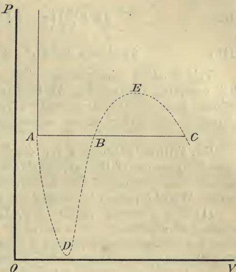
Fig. 18 (after Clausius).
