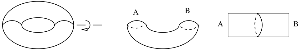
Figure 8. Visualizing the degree two map from E to E/\eta \cong \widehat{\mathbb{C}} , where \eta(z) = -z .
