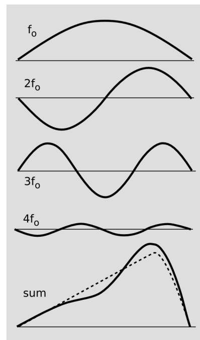
s / Using the sum of four sine waves to approximate the triangular initial shape of a plucked guitar string.
