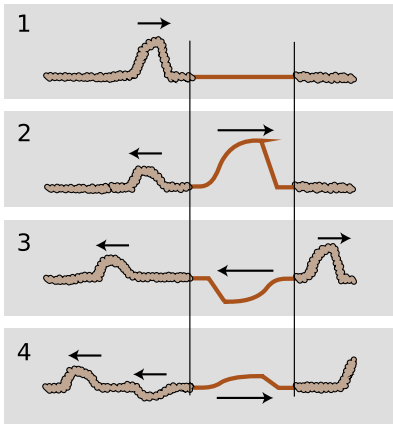
m / A rope consisting of three sections, the middle one being lighter.
