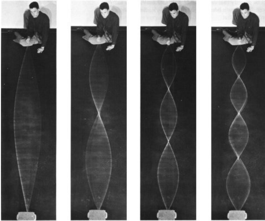
u / Standing waves on a spring.
