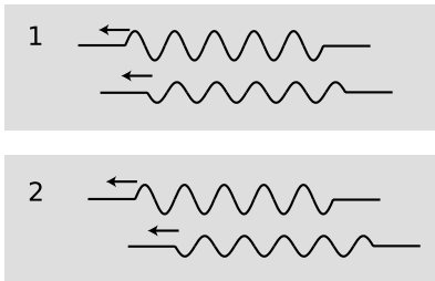
n / Two reflections, are superimposed. One reflection is inverted.
