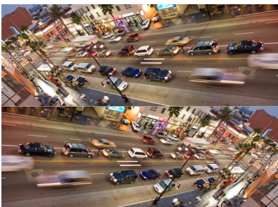
k / In the mirror image, the areas of positive excess traffic density are still positive, but the velocities of the cars have all been reversed, so areas of positive excess velocity have been turned into negative ones.
