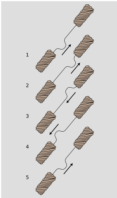
q / The motion of a pulse on the string.
