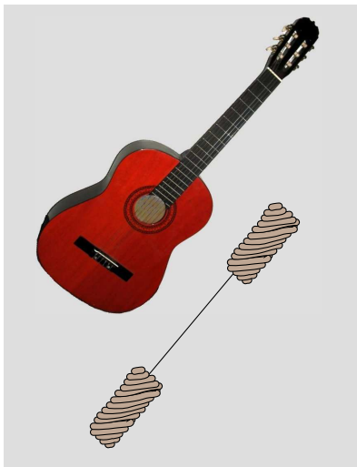
p / A model of a guitar string.
