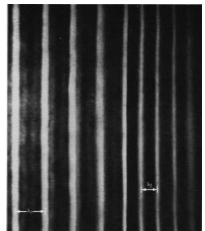
u / A water wave traveling into a region with a different depth changes its wavelength.
