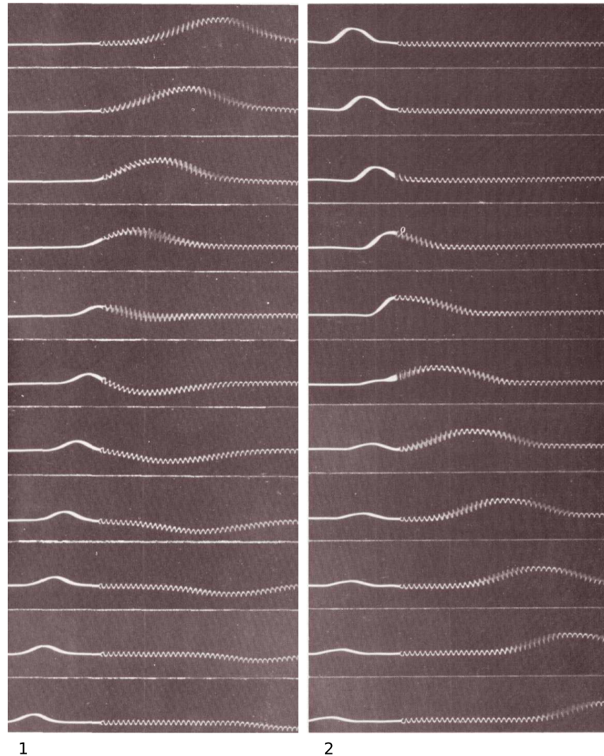
d / 1. A wave in the lighter spring, where the wave speed is greater, travels to the left and is then partly reflected and partly transmitted at the boundary with the heavier coil spring, which has a lower wave speed. The reflection is inverted. 2. A wave moving to the right in the heavier spring is partly reflected at the boundary with the lighter spring. The reflection is uninverted.
