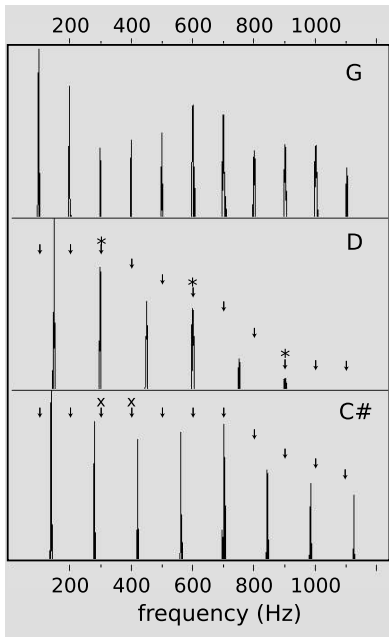
t / Graphs of loudness versus frequency for the vowel “ah,” sung as three different musical notes. G is consonant with D, since every overtone of G that is close to an overtone of D (*) is at exactly the same frequency. G and C# are dissonant together, since some of the overtones of G (x) are close to, but not right on top of, those of C#.
