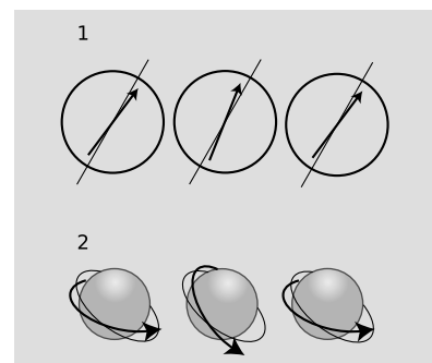
h / Example 14. 1. A compass needle vibrates about the equilibrium position under the influence of the earth's magnetic forces. 2. The orientation of a proton's spin vibrates around its equilibrium direction under the influence of the magnetic forces coming from the surrounding electrons and nuclei.
