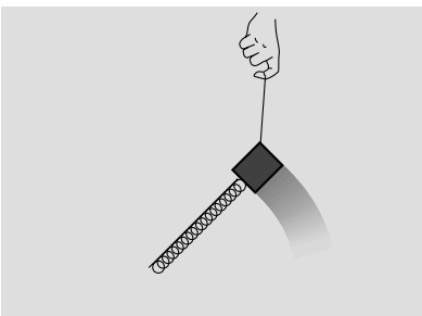
m / Driving at a frequency below resonance.
