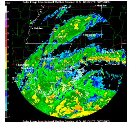
w / Example 8. A Doppler radar image of Hurricane Katrina, in 2005.
