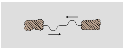
r / A tricky way to double the frequency.
