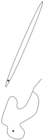
a / If we try to draw a non-repeating orbit for Halley's Comet, it will inevitably end up crossing itself.
