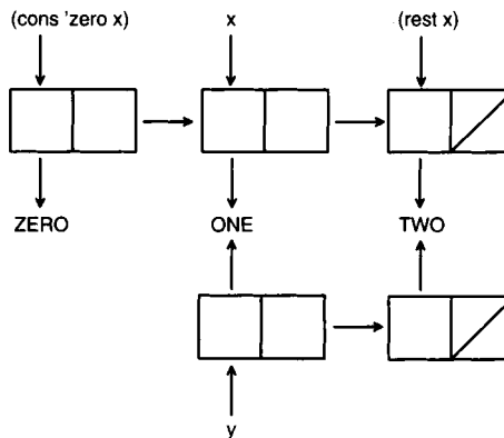
Figure 3.3: Parts of Lists
