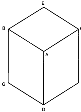
Figure 17.6: A Cube
