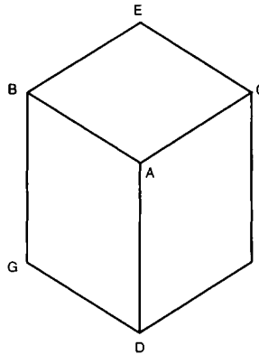
Figure 17.1: A Cube
