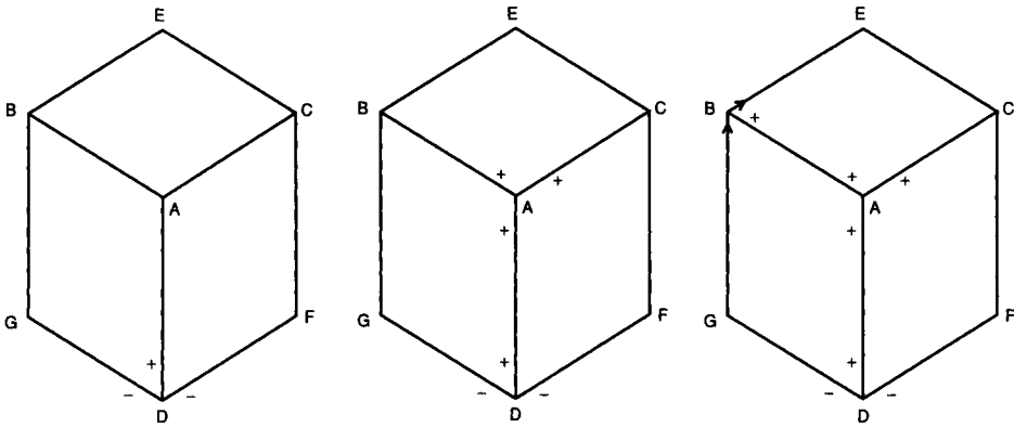
Figure 17.4: Propagating Constraints
