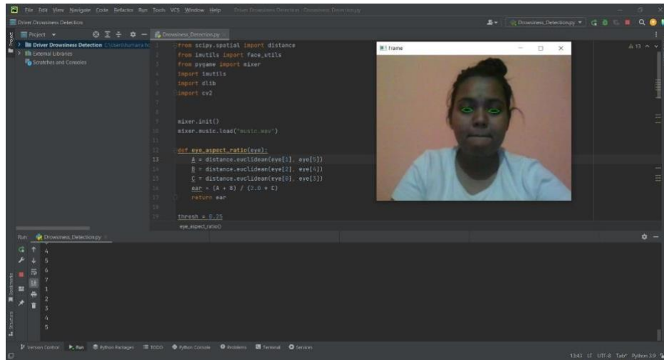
Figure 20: Fail Negative Mouth Detection
