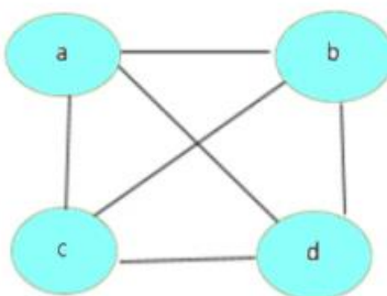
Fig. 5: Complete graph
