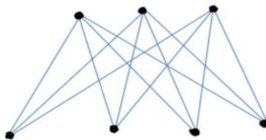
Fig. 8: Bipartite graph
