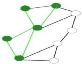
Fig. 4: Open walk (green highlighted)
