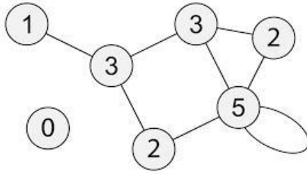
Fig. 2. Vertex degree representation
